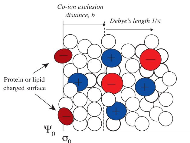
Fig. 5. A snapshot (possibly on a 0.1–0.01 \mu\text{s} ‘exposure’) of the Maxwellian double layer. The new feature is the appearance of the co-ion exclusion distance b , which separates the Debye–Hückel ionic cloud (characterized by the Debye’s length 1/\kappa ) from the surface charge \sigma_0 . The range of electrostatic forces is the sum of the co-ion exclusion distance and the Debye’s length.
