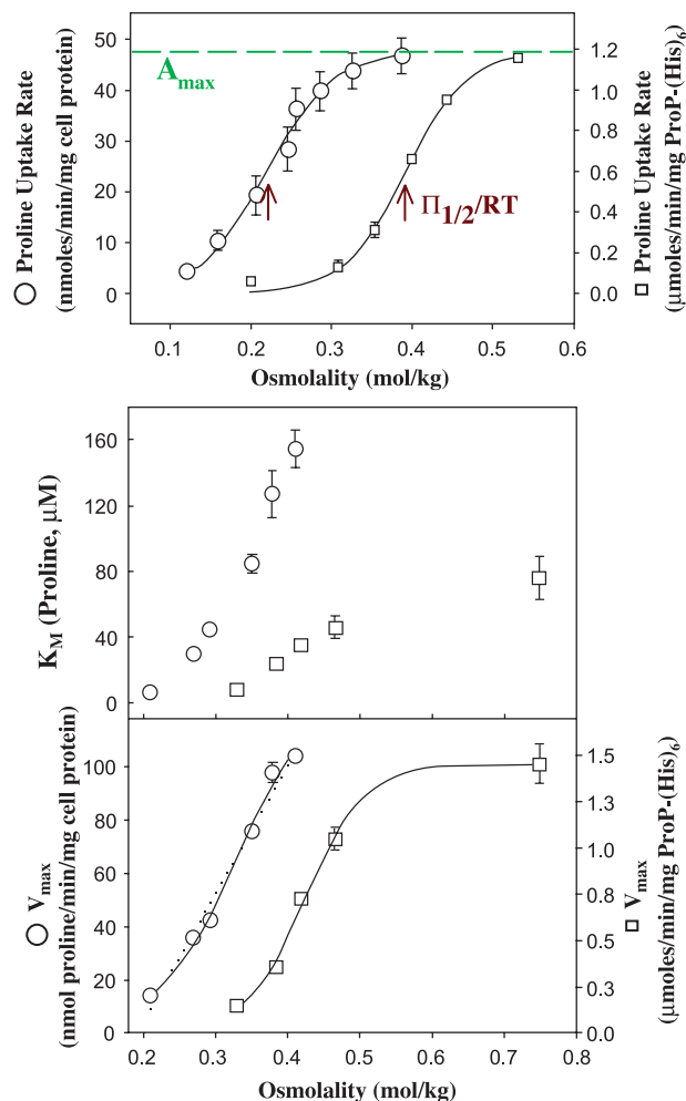
Fig. 3. Osmotic activation of ProP. Top: The initial rate of proline uptake via ProP-(His) 6 is a sigmoid function of external osmolality in bacteria (circles) and in proteoliposomes prepared with E. coli lipid and the pure protein (squares). Transporter function can be characterized in terms of the activity approached at high osmolality ( A_{\text{max}} ), the osmolality required to attain half that maximal activity ( \Pi_{1/2}/RT ) and the gradient of the osmolality response (B). Middle: The apparent K_M of ProP for proline is a direct function of osmolality in both bacteria (circles) and proteoliposomes (squares). The absolute values of K_M for these two systems differ, however. Bottom: ProP is activated at different osmolalities in bacteria and in proteoliposomes even if the osmolality dependence of K_M is taken into account. Reprinted with permission from Culham et al. [46]. Osmosensor ProP of Escherichia coli responds to the concentration, chemistry and molecular size of osmolytes in the proteoliposome lumen [46]. Copyright 2003 American Chemical Society.
